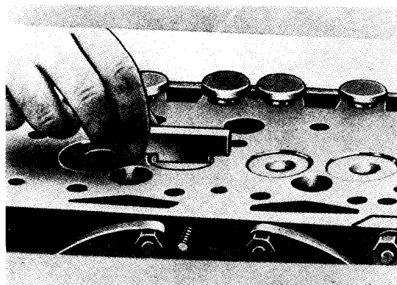
Sl. 2B.8 — Provera upadanja ventila
